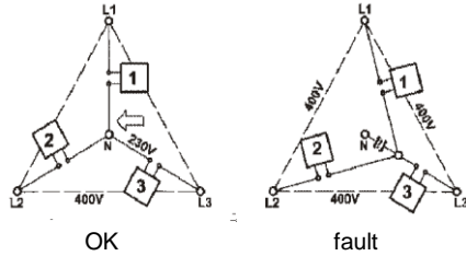
Light fittings with emergency light unit
