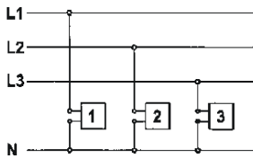
Light fittings with emergency light unit
